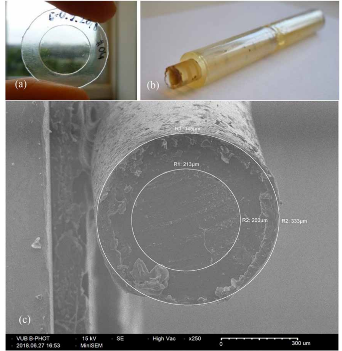
Fig. 4. (a) Photograph of the compression molded PDLGA sheet, (b) Photograph of the preform (P2) consisting of a PDLGA rod inserted into a PDLA tube. Yellowish discoloration was caused by thermal oxidation. (c) SEM image of the eventual step-index bioPOF, with a core-cladding ratio of about 4:7, where the core radius is around 213–200 \mu\text{m} and the cladding radius is 345–333 \mu\text{m} .
