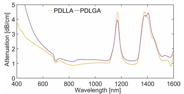
Fig. 1. Attenuation expressed in dB/cm of flat PDLGA and PDLGA sheets fabricated using compression molding.
